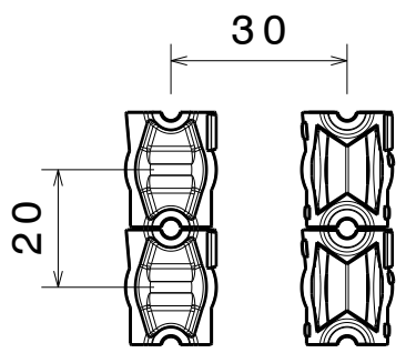
Strada lens arrangement recommendation
