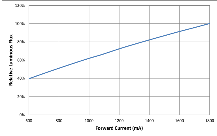
Relative Output Flux vs. Forward Current @ 100°C
