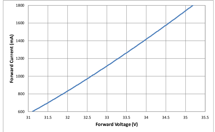
Forward Current vs. Forward Voltage @ 100°C
