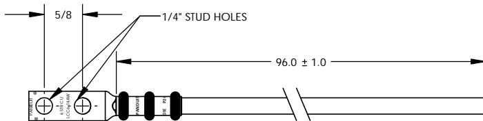
FACTORY CRIMPED #6 AWG/16mm SQ. JUMPER WIRE ASSEMBLY (QTY. 1) INCLUDES: LCC6-14AW (QTY. 1) #6 AWG/16mm SQ. WIRE - GREEN/YELLOW INSULATION 96" LONG
